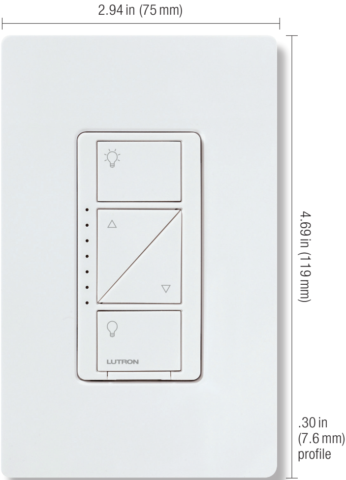
Shown actual size: Caséta Wireless in-wall dimmer and 1-gang Claro wallplate in White (WH).
