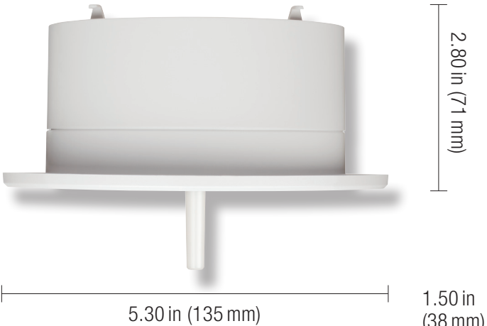
Shown: Vive wireless hub and flush-mount adapter
