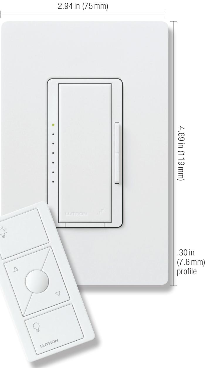
Shown actual size: Vive Maestro Wireless dimmer and 1-gang Claro wallplate in White (WH). Shown actual size: Pico wireless remote in White (WH), W: 1.25 in (31.75 mm) x H: 2.63 in (66.80 mm) x D: .33 in (8 mm).
