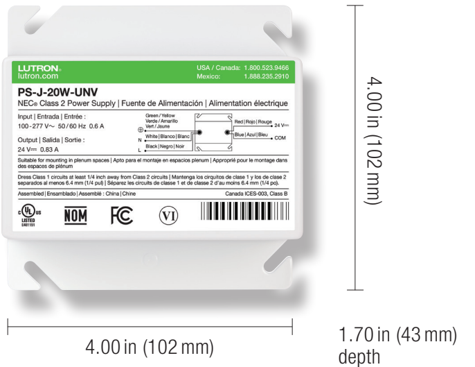
Shown: Vive wireless hub external power supply
